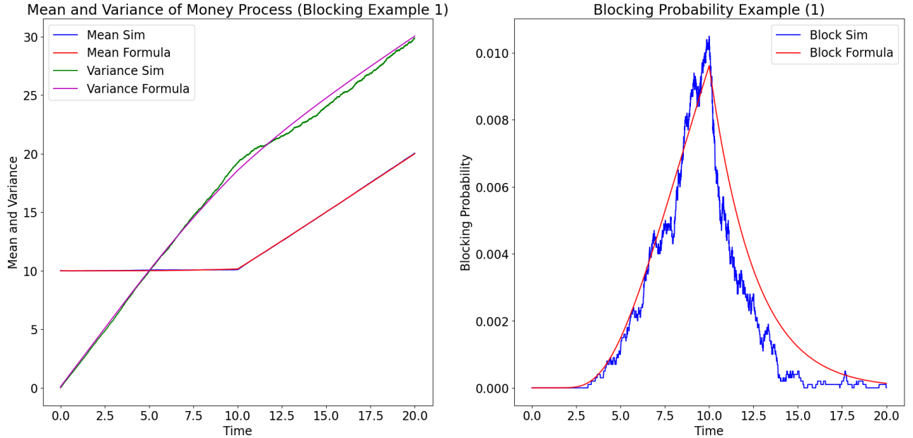
Figure 4: Mean and Variance of the Blocking Money Process (left) and blocking probability (right) for Example 1.
