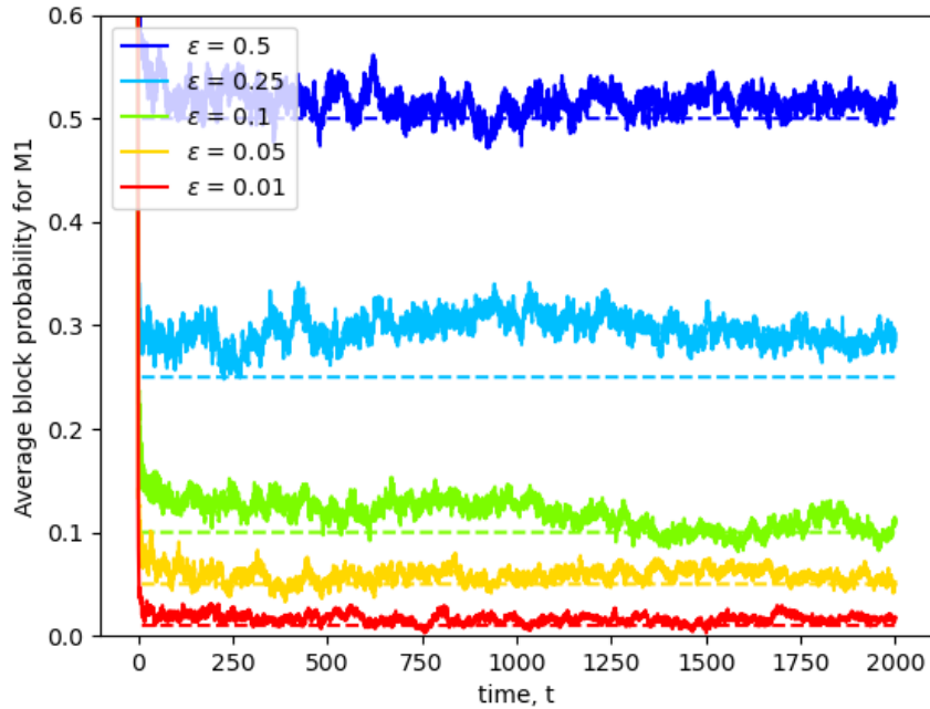
Figure 6: Stabilizing the probability of blocking for \varepsilon \in \{0.01, 0.05, 0.1, 0.25, 0.5\} .
