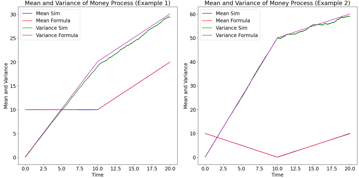
Figure 3: Mean and Variance of the Bail Everyone Out Money Process
